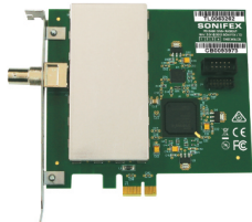
The PC-FM6-32 FM Radcap PCIe Card (6 to 32 Channels)
